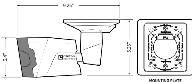
MOUNTING PLATE
