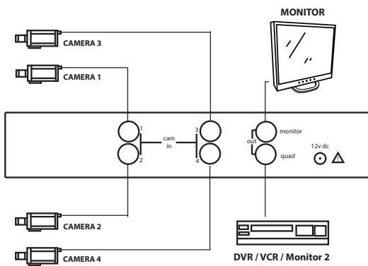
Rear Panel
